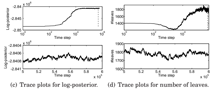
Fig. 9. The 2D-Gaussian density and its resulting posterior mean histogram estimate with 6022 boxes with IAE = 0.0502. The starting state has 1404 leaf nodes. Burnin is taken at time step 500000 and 10000 samples are collected with a thin-out of 10.
