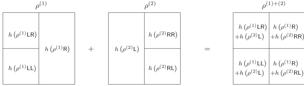
Fig. 4. Adding two SRP histograms.
