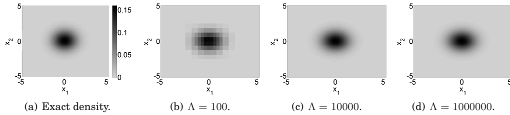
Fig. 6. 2D-Gaussian: Plots of the exact density and its approximations with \Lambda = 100, 10000, 1000000 .
