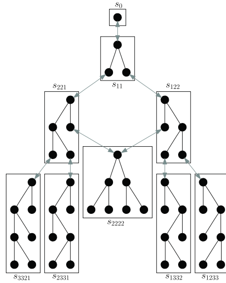
Fig. 2. Transition diagram over S_{0,3} with split/reunion transitions from one RP state to another.
