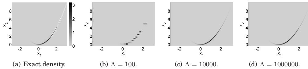
Fig. 7. 2D-Rosenbrock: Plots of the exact density and its approximations with \Lambda = 100, 10000, 1000000 .
