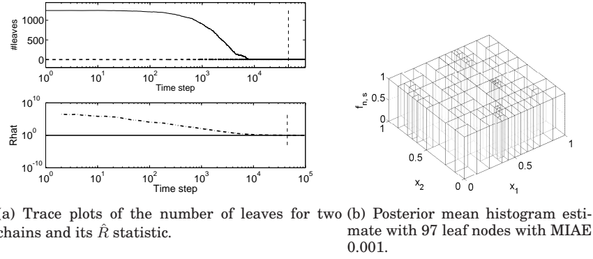
Fig. 5. A typical run of two Metropolis-Hastings chains based on 10^6 data points from the 2D-uniform density. The chains have been started from the root node and a state with 1247 leaf nodes. 10000 histogram samples were collected with a thin-out of 10 after burn-in at time step 44861.
