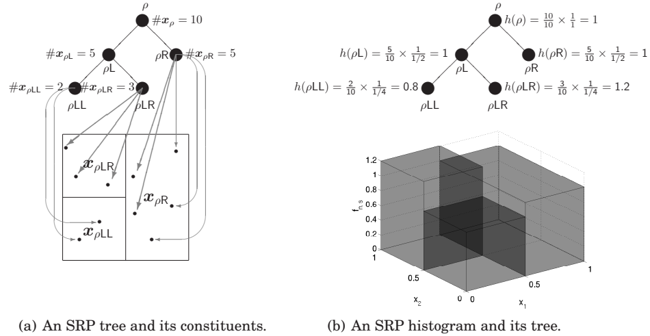
Fig. 3. An SRP and its corresponding histogram.
